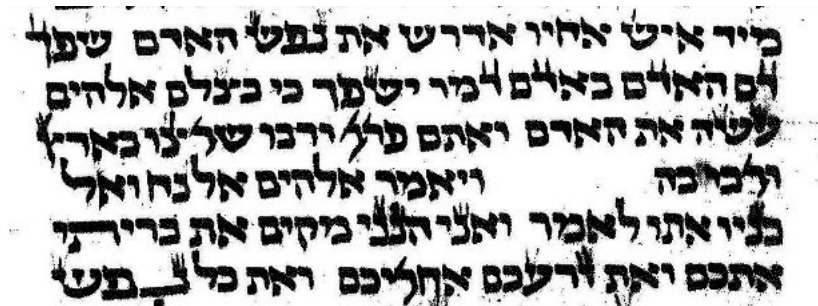
Abb. 19: BSB 488 (Gen 9,6–9)
